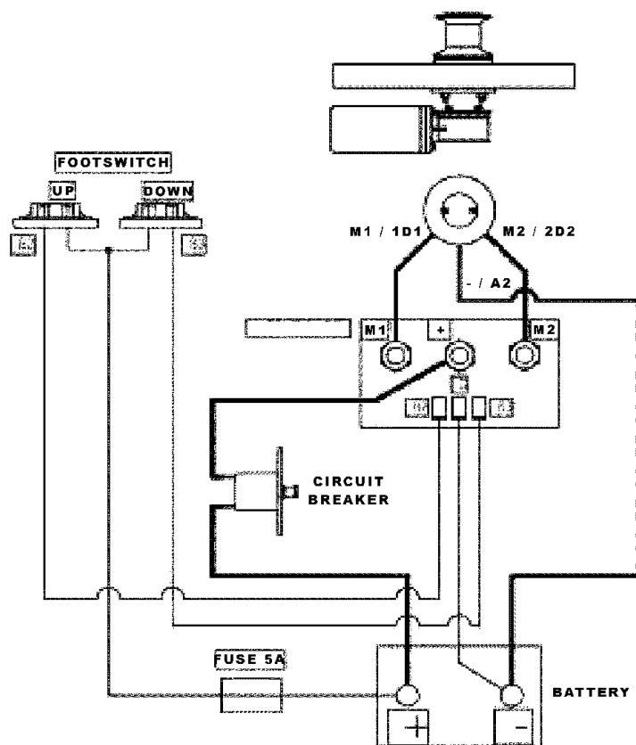
3 TERMINAL MOTORS
